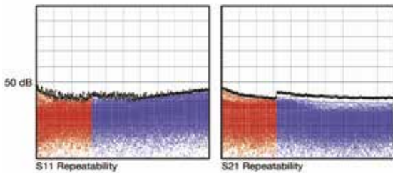
Repeatability for XT981ML01 Multi-Harmonic automated tuners (repeatability response for individual probes).
